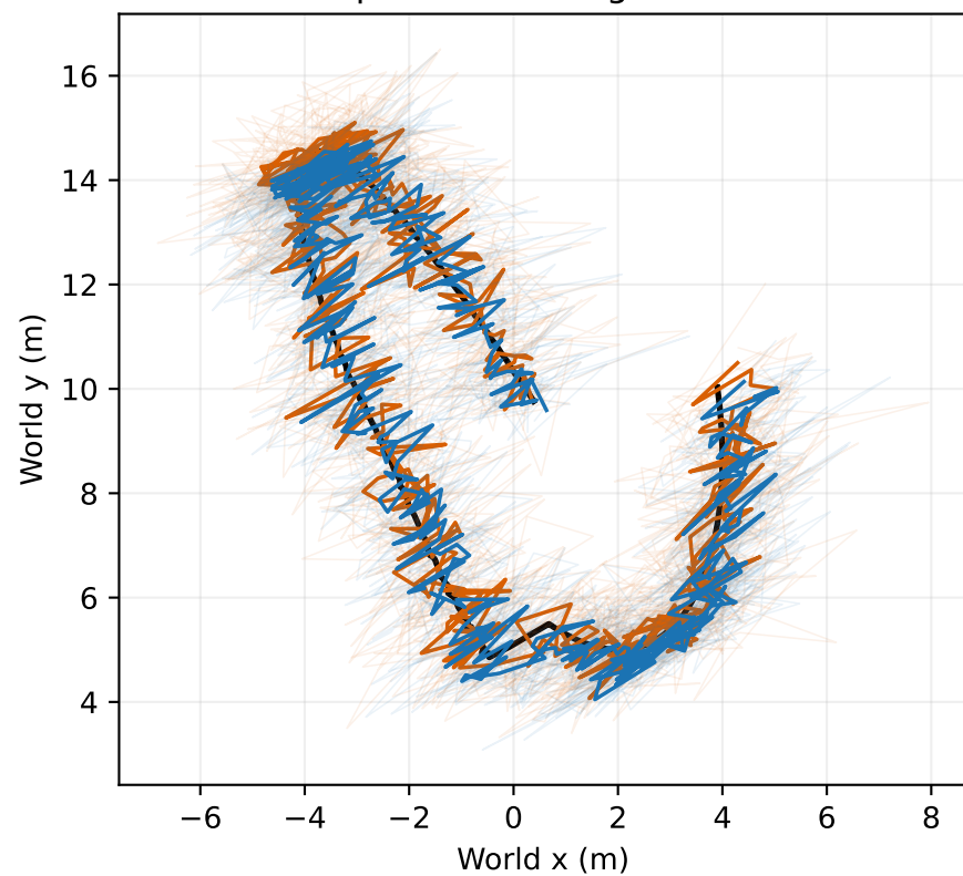
seq07: 3D RMSE gain 7.9%
