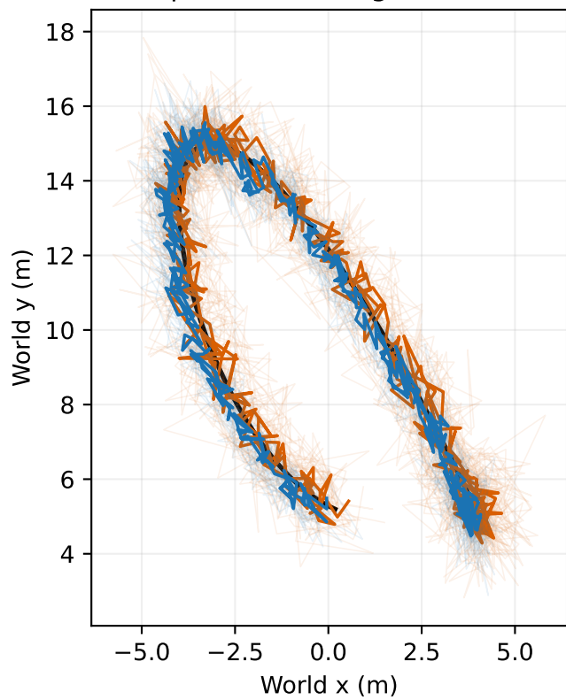
seq10: 3D RMSE gain 10.7%
