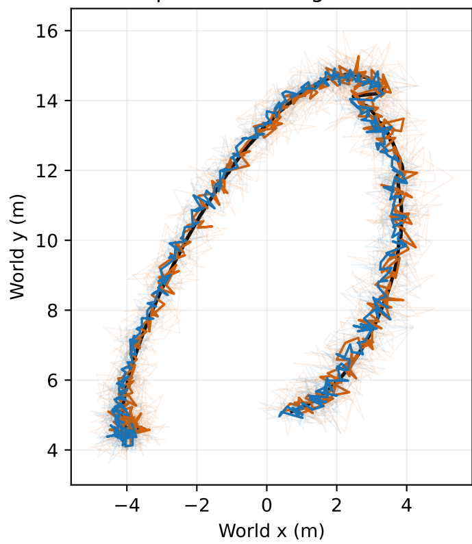
seq10: 3D RMSE gain 10.7%
