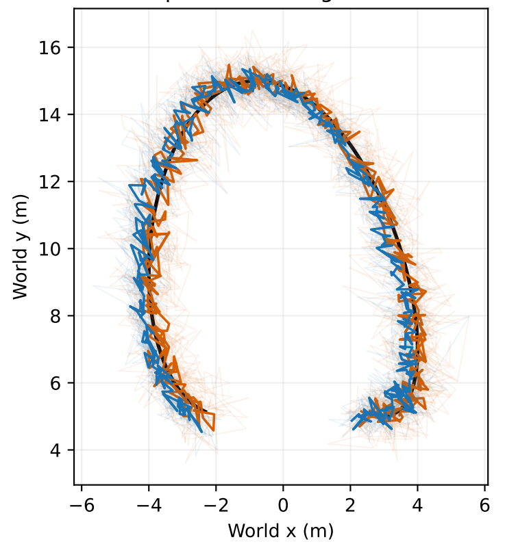
seq11: 3D RMSE gain 9.4%
