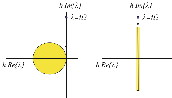
Fig. 4.1 Stability regions for Euler's method ( left ) and Symplectic Euler/Verlet ( right ). When a harmonic oscillator is treated using these methods, the origin is unstable for Euler's method, regardless of stepsize—this means that there is no choice of scaling h which will allow us to ensure that |1 + h\lambda| \leq 1 . On the other hand, the Verlet method has an interval of stability on the imaginary axis, and it is always possible to find a value of h which guarantees that |h\Omega| \leq 2
