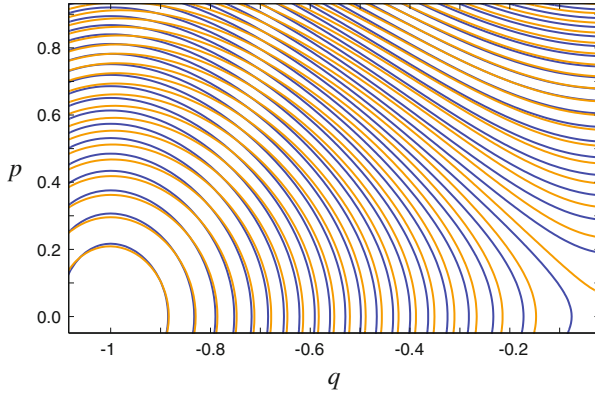
Fig. 3.3 The isoenergy contours are shown for the double well model ( dark curves ) together with the corresponding curves for the Verlet modified Hamiltonian ( light curves )
