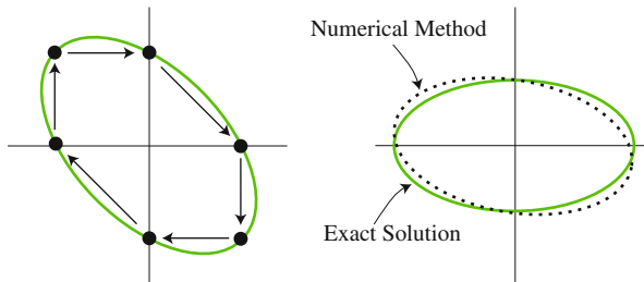
Fig. 3.1 Numerical solutions of the harmonic oscillator may cycle through a finite number of discrete points ( left ) or may gradually fill in an ellipse that is just a slight perturbation of the correct energy level set ( right )
