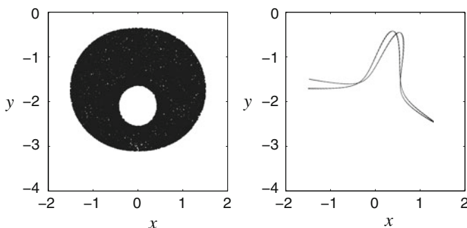
Fig. 3.14 The steady state behavior obtained in the pendulum example using Verlet ( left ) and the projected Verlet method ( right ). The graphs show the final 450,000 steps of simulation in a 500,000 step trajectory
