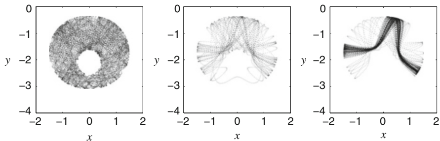
Fig. 3.13 A projected Verlet trajectory for the pendulum model is shown in its xy projection for three successive intervals of timesteps (see text for discussion). The graphs show the transition from correct sampling behavior to motion confined to a limit cycle
