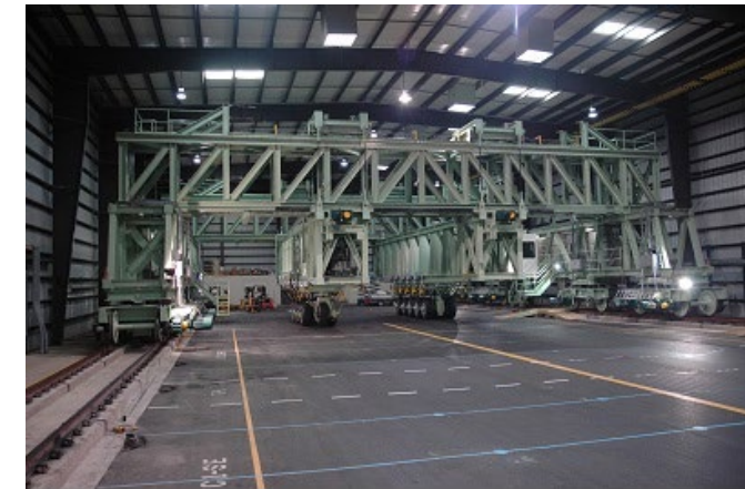
The National Airport Pavement Test Vehicle
