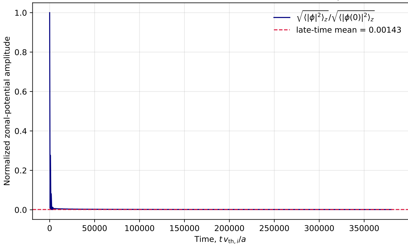
Rosenbluth--Hinton zonal-flow relaxation: k_x = 0.05 , k_y = 0
