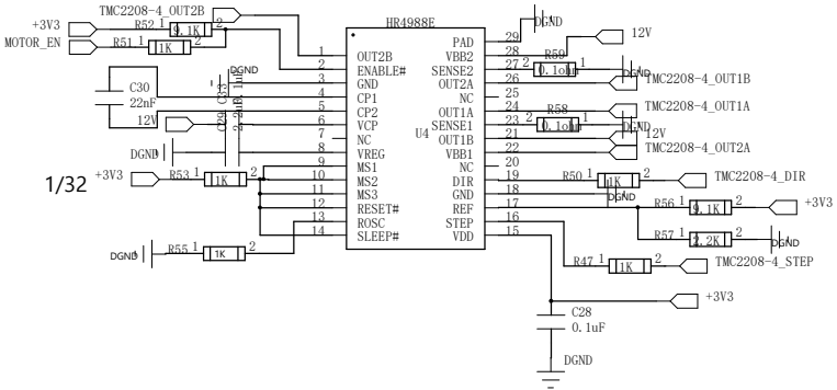
驱动芯片：HR4988
