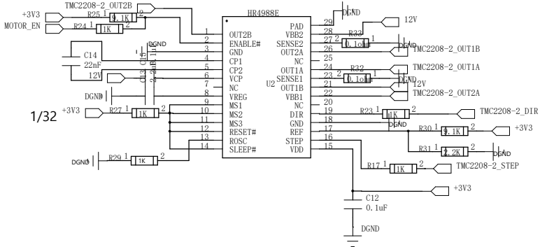
驱动芯片：HR4988
