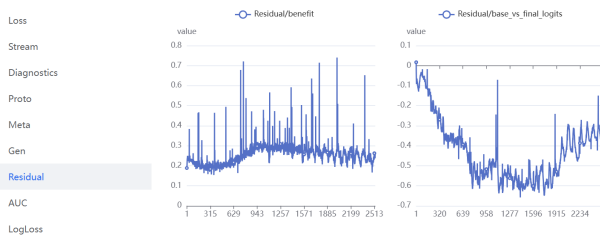
Figure 6: Residual path validation. Left: residual benefit stabilizes at 0.2–0.3; Right: base_vs_final_logits drifts to -0.4 , indicating conservative residual correction.
