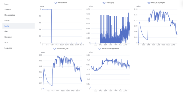
Figure 3: MetaAligner dynamics. Top-left: mode transition from fast (1) to stable (0); Top-middle: train-valid AUC gap \bar{g} ; Top-right: auxiliary weight \lambda_{\text{aux}} ; Bottom-left: EMA of auxiliary weight; Bottom-right: residual benefit \bar{r} . The gap expansion triggers conservative \lambda_{\text{aux}} suppression, yet residual benefit remains positive.
