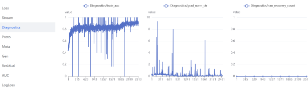
Figure 7: Numerical stability diagnostics. Left: train AUC; Middle: CTR gradient norm (spikes auto-masked); Right: NaN recovery count remains zero throughout training.
