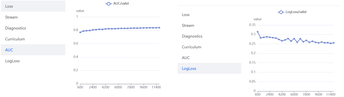
(b) Validation AUC of the ablated variant. Despite training instability, the validation AUC improves monotonically from 0.78 to 0.83, confirming that the core principle of sequence-parameterized cross-field interaction remains effective even when the optimal-transport machinery is removed.
