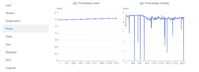
Figure 4: Prototype health metrics. Left: concentration \kappa stable at \sim 1.8 ; Right: assignment entropy stable at 4.3 (89% of maximum), indicating informative soft semantic IDs.
