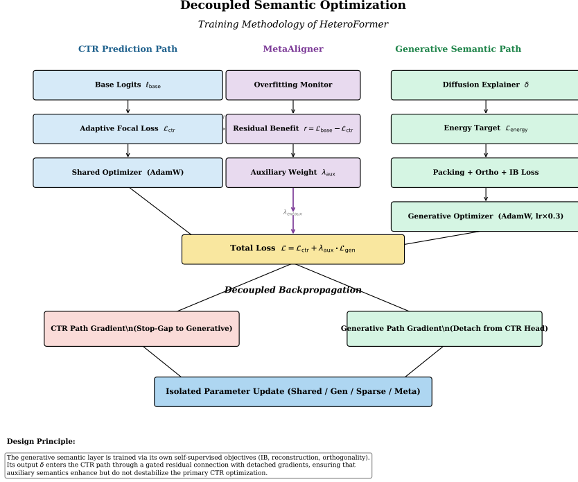
Figure 2: Decoupled Semantic Optimization. The CTR path and Generative Semantic path share forward computation but receive isolated gradients. MetaAligner modulates the coupling weight \lambda_{\text{aux}} based on residual benefit and overfitting gap.
