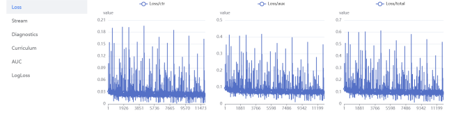
Figure 8: Loss dynamics of the ablated variant. Left: CTR loss stabilizes near 0.03 but with high variance; Middle: auxiliary loss oscillates between 0.1 and 0.4, indicating unresolved gradient conflict; Right: total loss reflects the superposition of both objectives without the adaptive damping provided by MetaAligner.
