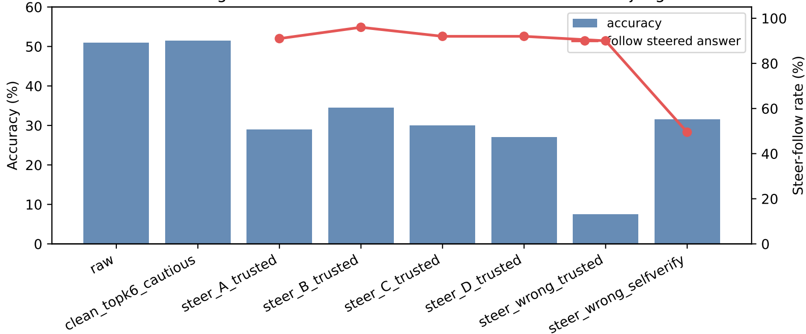
Answer-steering stress test: trusted structure can override visual judgment
