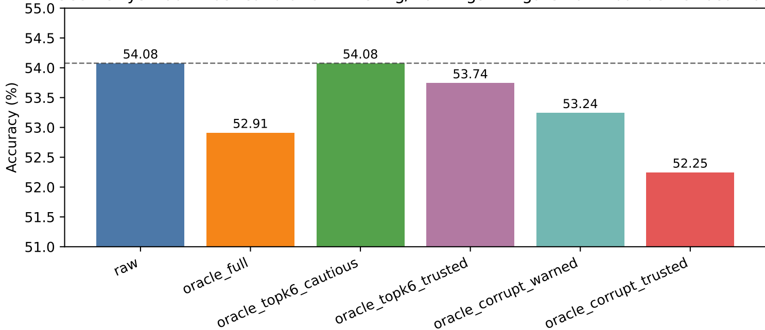
Geometry3K-601 trust calibration: filtering/warnings mitigate harm but do not beat raw
