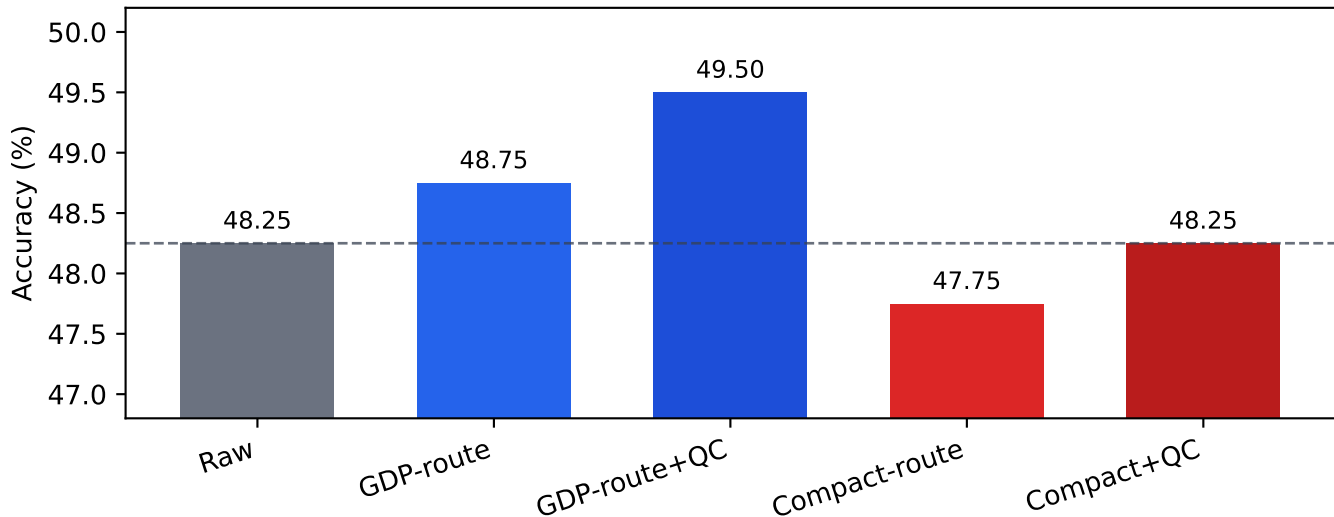
Cross-dataset GDP-route validation (PGPS9K 200 + Geometry3K 200)
