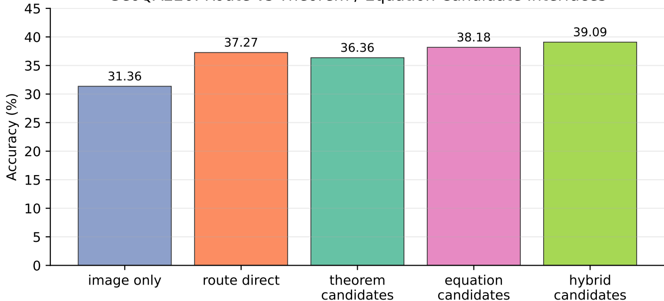
GeoQA220: Route vs Theorem / Equation Candidate Interfaces
