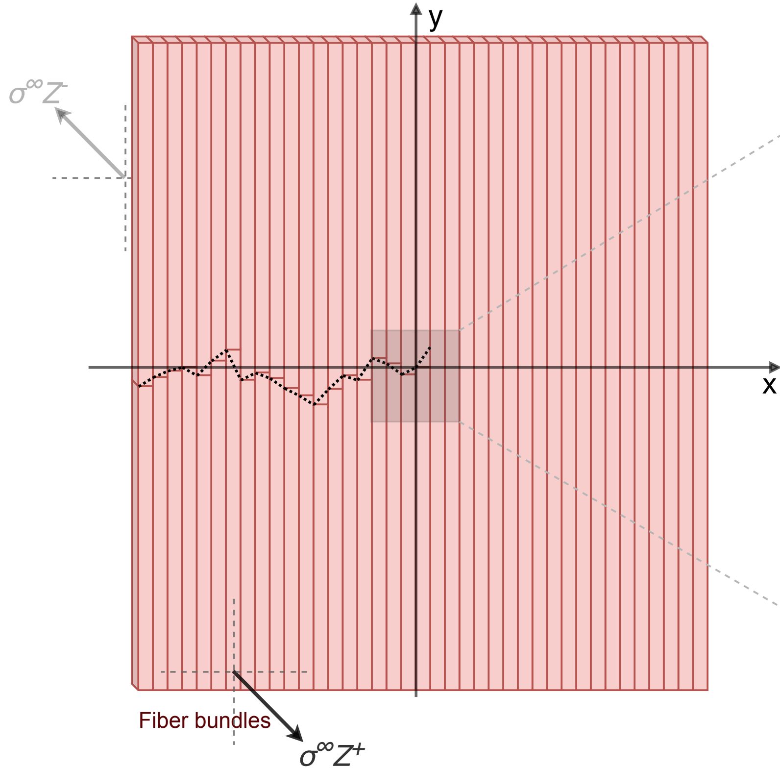
a Bamboo microstructure and fracture propagation
