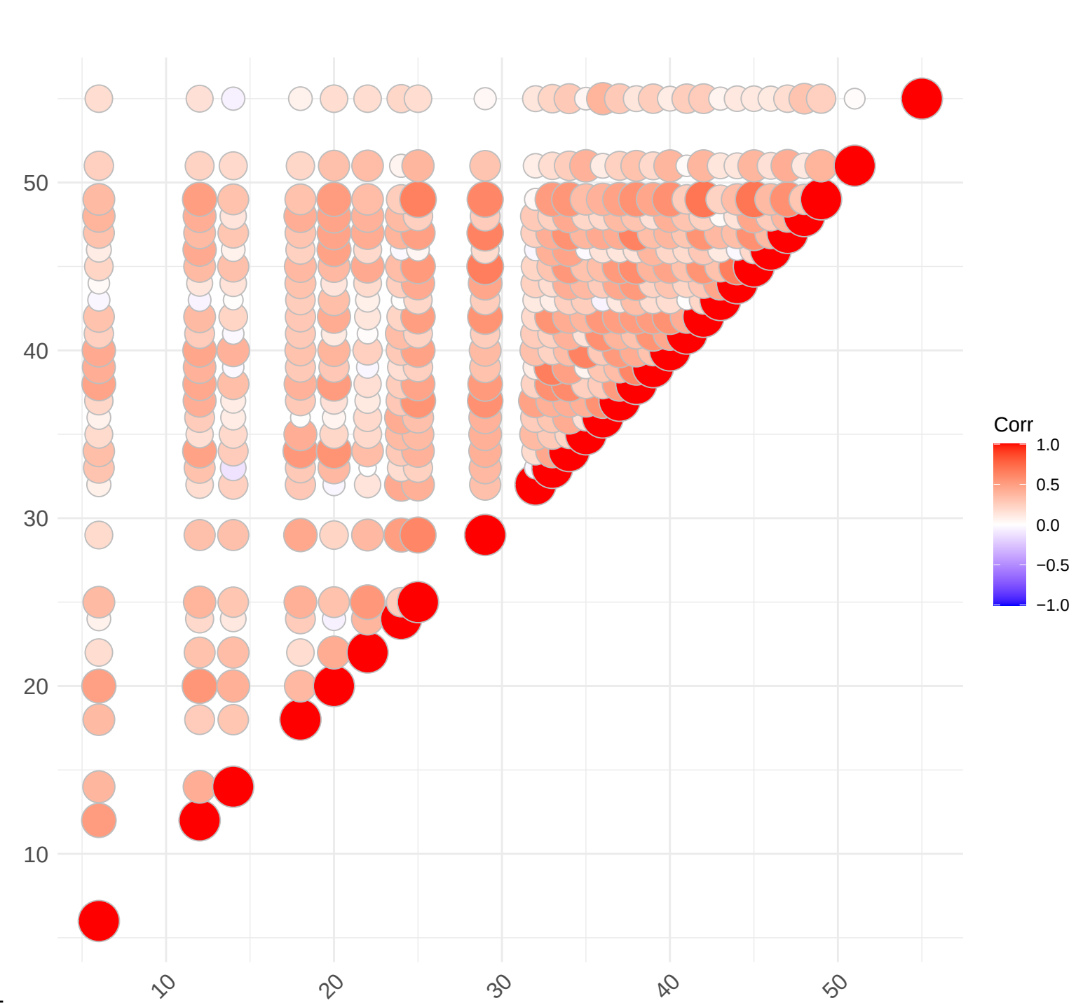
Leucoraja_erinacea_little_skate
