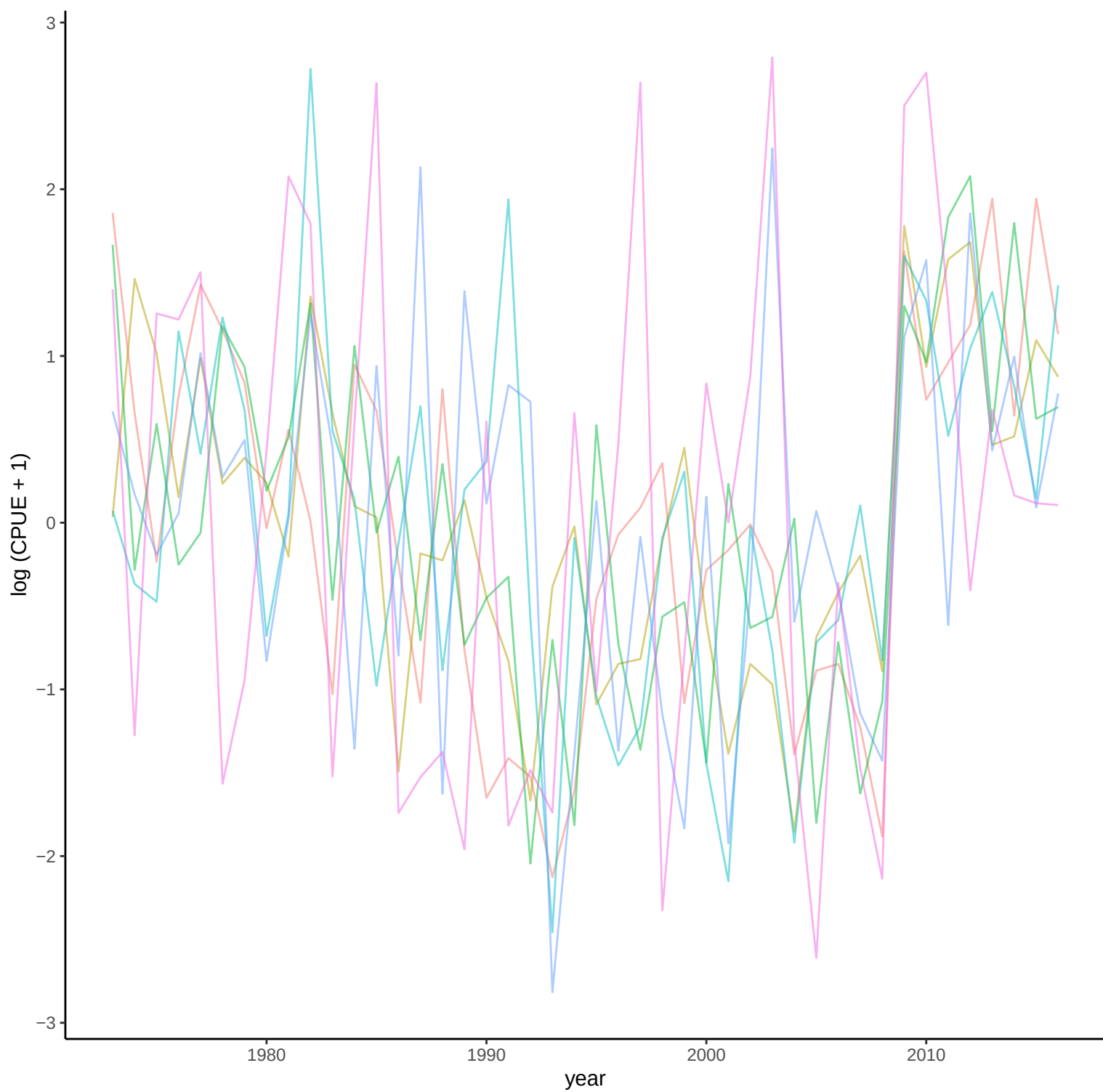
Leucoraja_erinacea_little_skate
