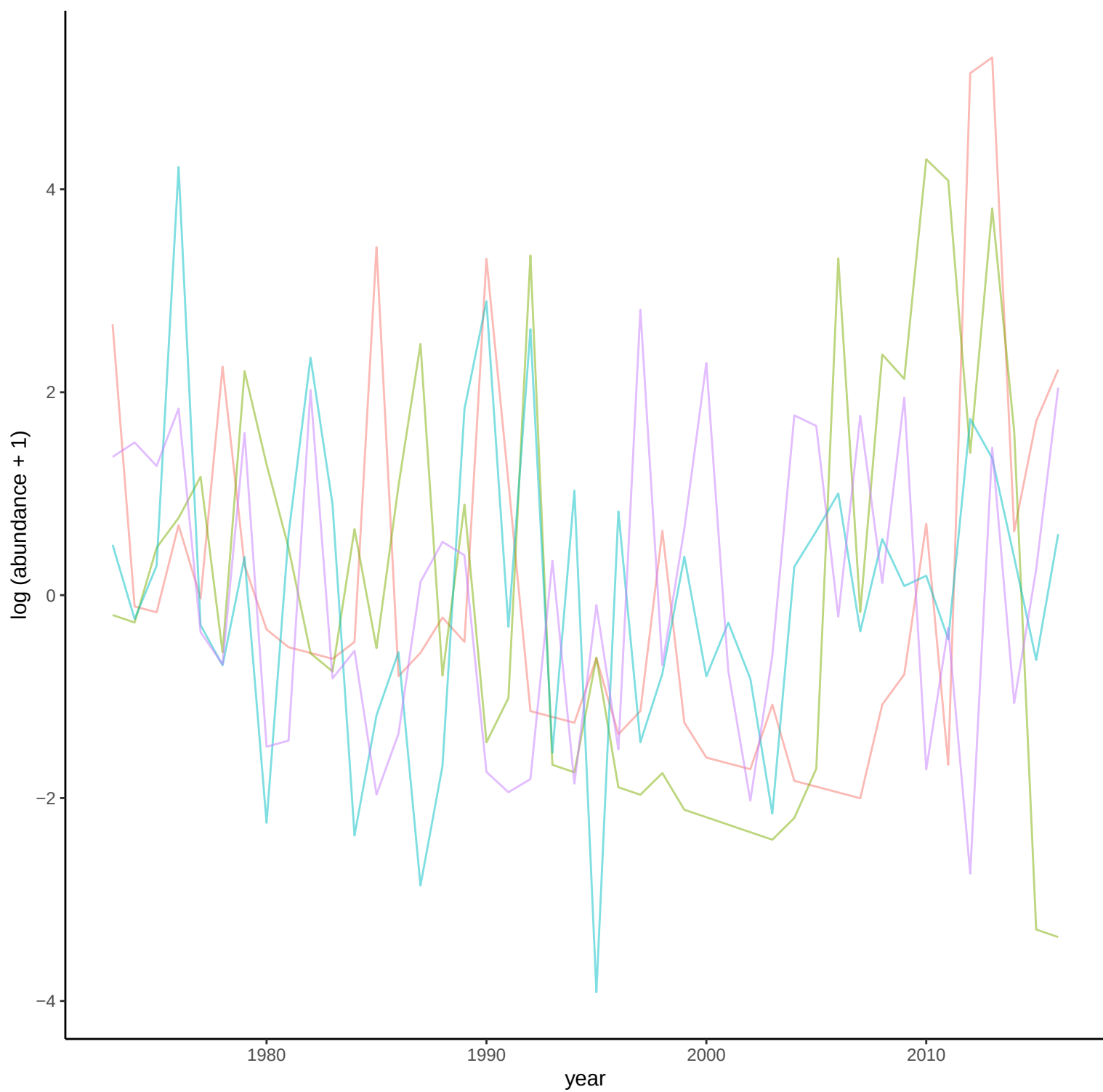
Squalus acanthias _spiny_dogfish
