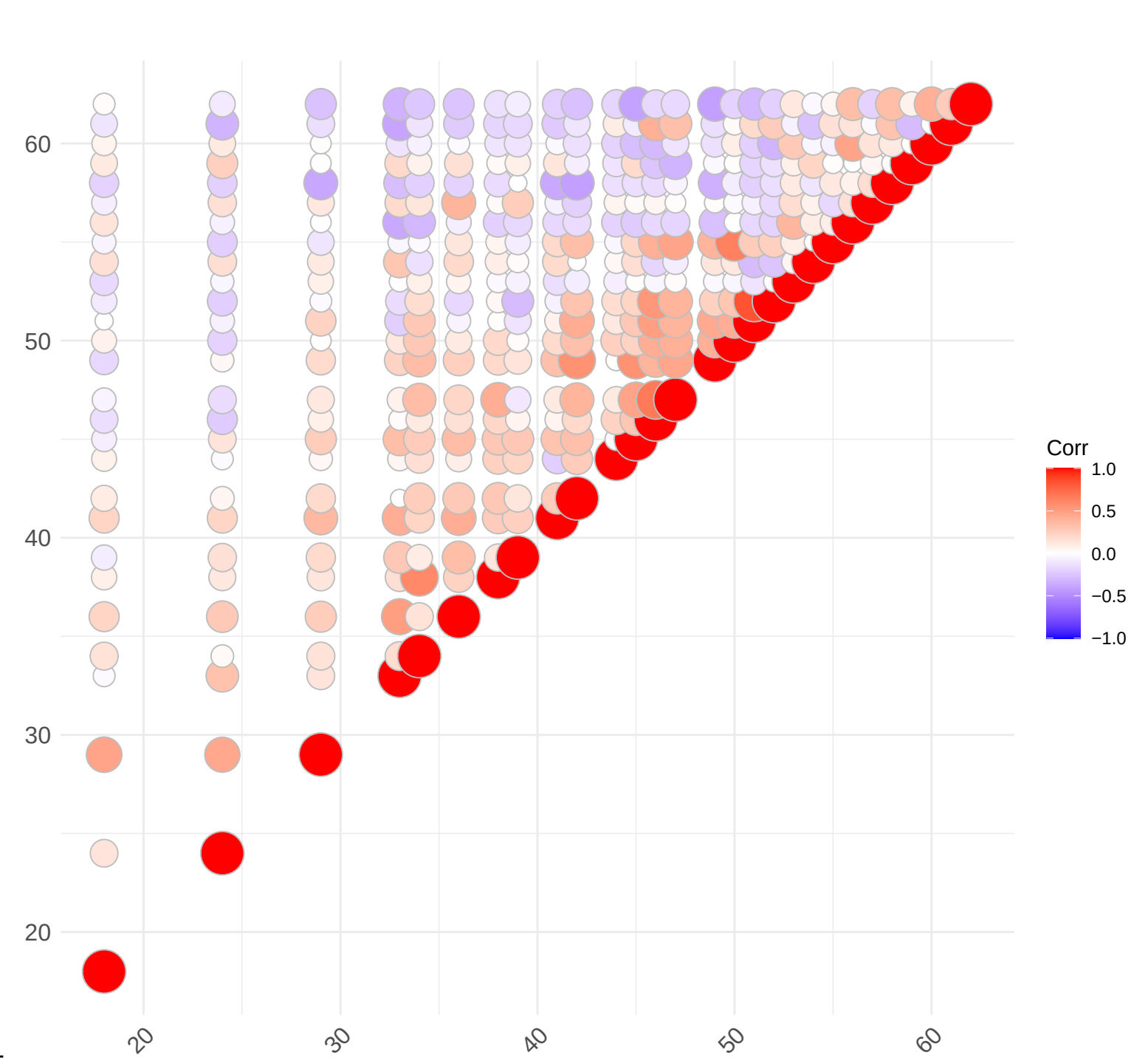
Squalus acanthias _spiny_dogfish
