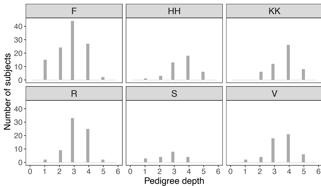
Figure S1. Distribution of pedigree depth for the 347 subjects from the six social groups.
