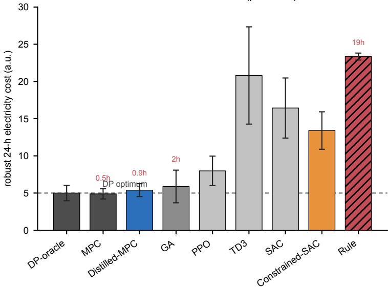
Gun-barrel — robustness (perturbed)
