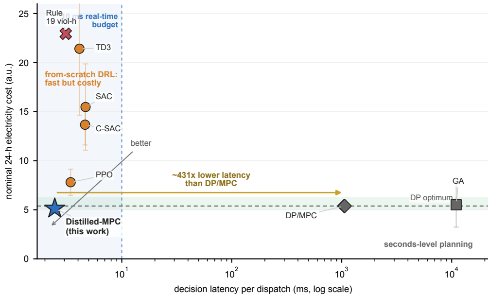
Fig. 11 | Cost-latency Pareto map
