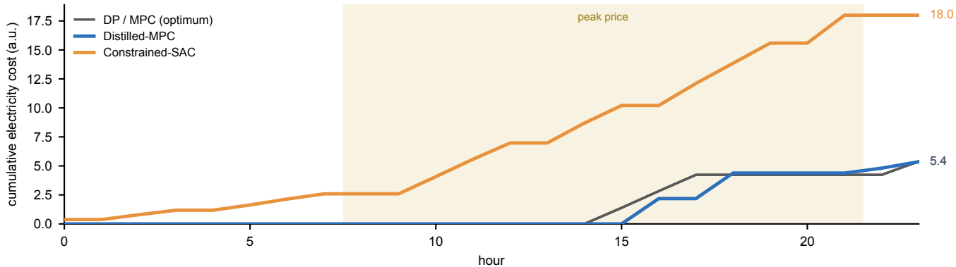
a Distilled-MPC tracks the DP/MPC optimum; Constrained-SAC spends ~3× more
