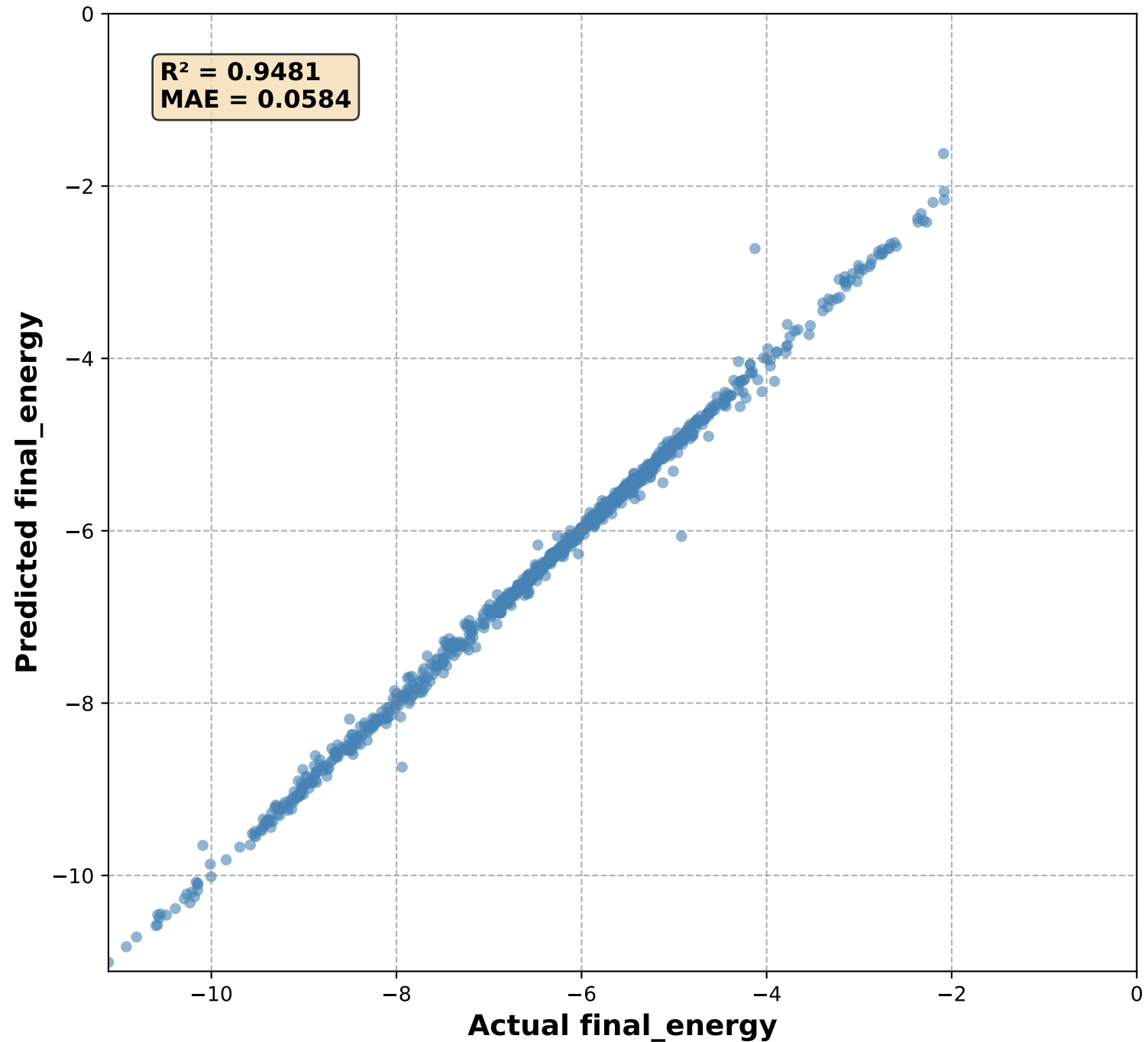
Actual vs Predicted final_energy ( R^2 = 0.9481 , MAE = 0.0584)
