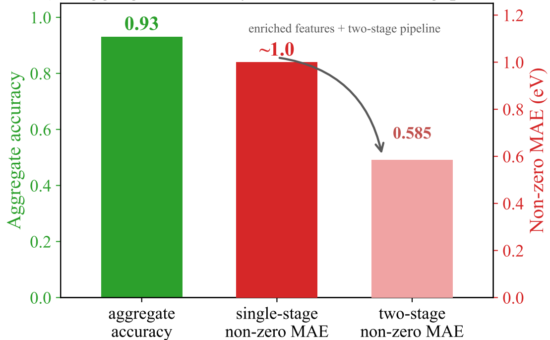
(a) Aggregate accuracy obscures non-zero-gap error
