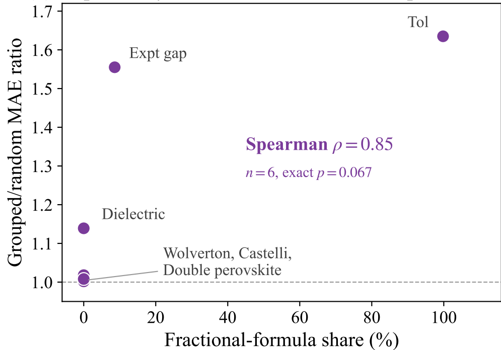
(b) Exploratory: fractional formulas and split sensitivity
