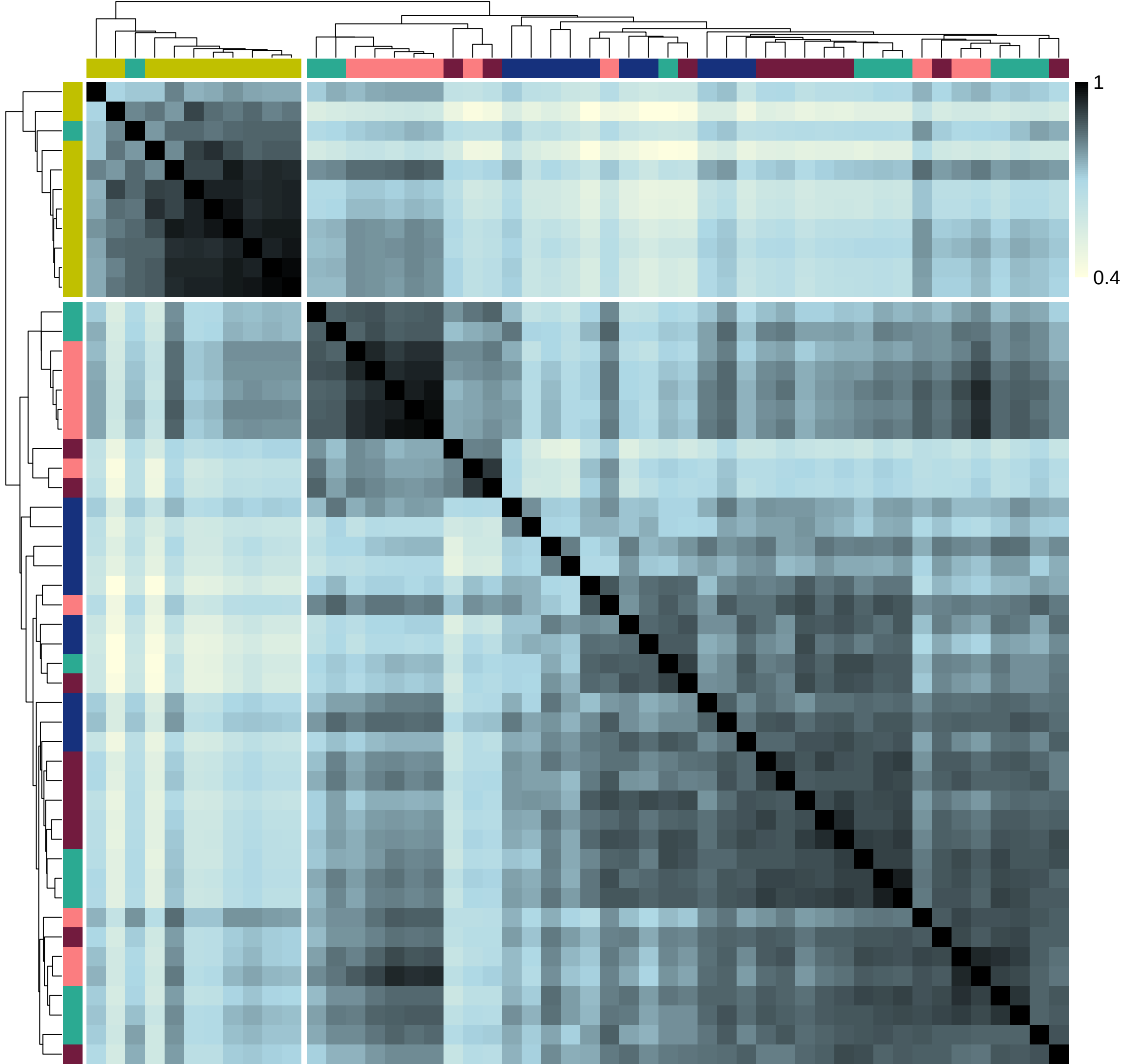
Spearman Similarity Heatmap
