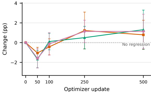
(b) Worst-domain change
