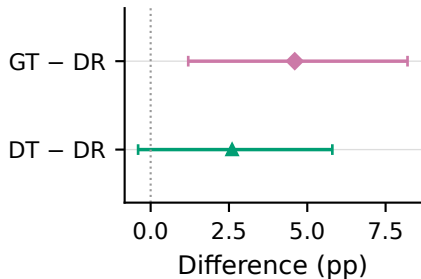
GPQA
