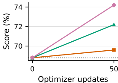
GPQA avg@4
