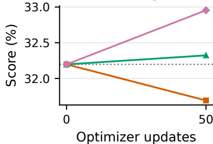
GPQA avg@4
