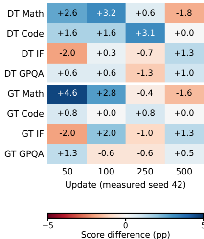
(c) Capability vs DR
