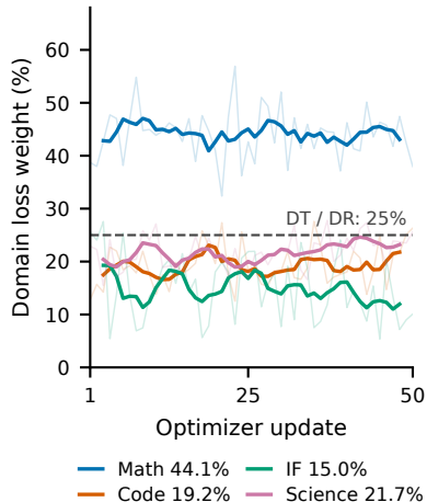
(a) Domain weights
