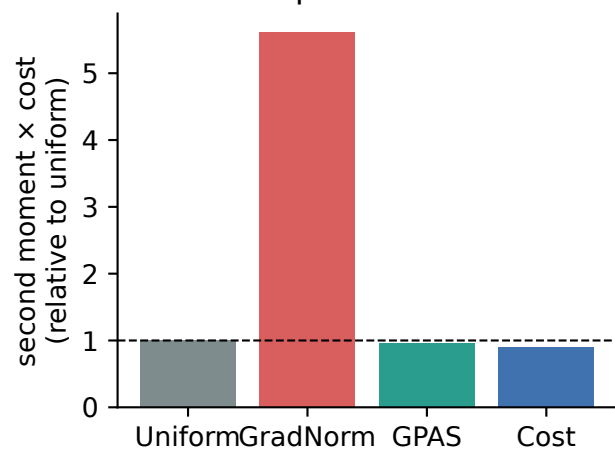
Compute criterion
