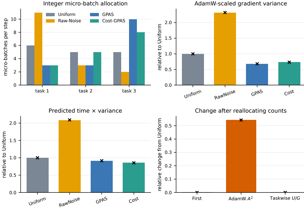
Figure 4: Controlled checks. Bars are Monte Carlo estimates and crosses are calculated values. GPAS uses AdamW-scaled within-task noise; Cost-GPAS also uses task cost. The last panel compares second-moment observations after an integer reallocation.
