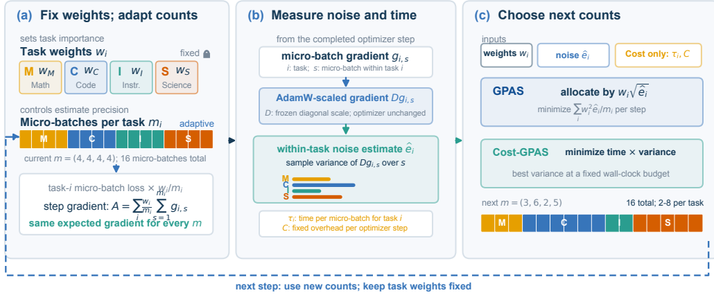
Figure 1: GPAS fixes the objective weights w and adapts only the micro-batch counts m . Gradients from the completed step give each task’s noise in AdamW coordinates, and measured time adds the cost correction, so the next allocation needs no additional model passes.
