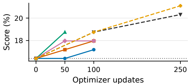
GPQA avg@4
