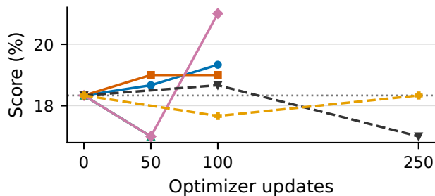
IFBench strict
