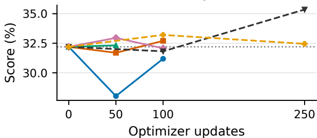
GPQA avg@4
