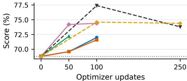
IFBench strict
