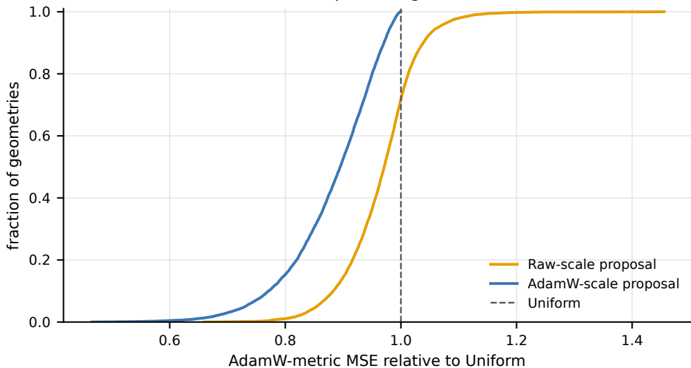
Random optimizer geometries
