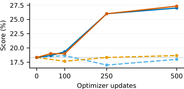
IFBench strict
