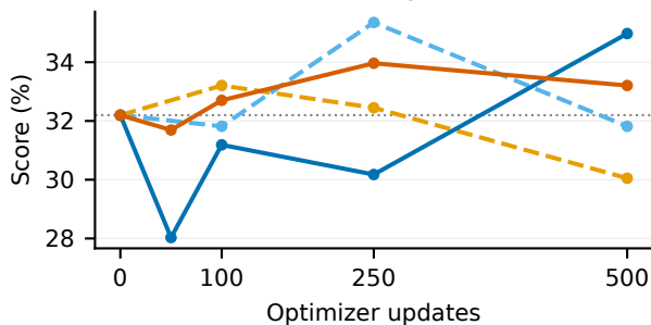
GPQA avg@4
