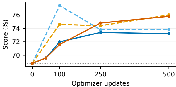
IFBench strict
