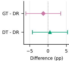
GPQA
