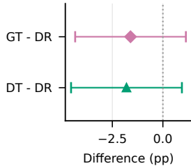
Math
