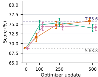
(c) MATH-500
