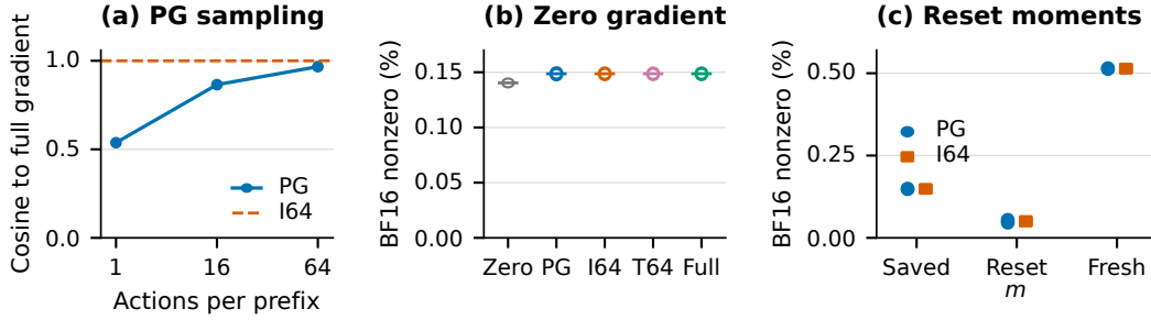
Figure 6: Averaging more token samples improves gradient alignment; Adam history contributes strongly to BF16 changes. (a) Gradient cosine to full-vocabulary supervision, using 12 fixed prefix subsets with two independent sampling repetitions per budget; I64 uses the top-64 intersection. (b,c) Fractions of changed BF16 weights with zero current gradient or reset moments. PG denotes sampled-token supervision; reset- m keeps the second moment and step count, and fresh Adam resets both moments and the count. Points show batches and bars show means.
