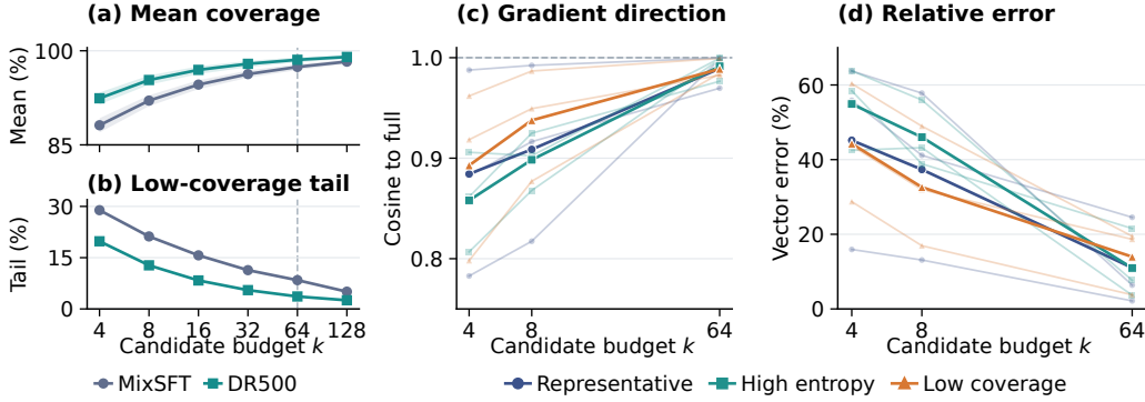
Figure 6: Larger candidate sets retain more probability mass and reduce gradient error in these comparisons. (a,b) Mean retained student probability and the fraction below 90%, using 384 responses per model; bands: response-cluster 95% intervals. Dashed lines mark k = 64 . (c,d) Gradient cosine and relative error against full-vocabulary KL at the same trained model (DR500). Colors distinguish typical inputs, uncertain next-token predictions, and inputs where I64 omits more probability mass. Thin lines show three batches per group; bold lines show group means. The reported I64 error range spans all nine batch values at k = 64 . Coverage and teacher targets use BF16 forwards; student gradients use FP32.
