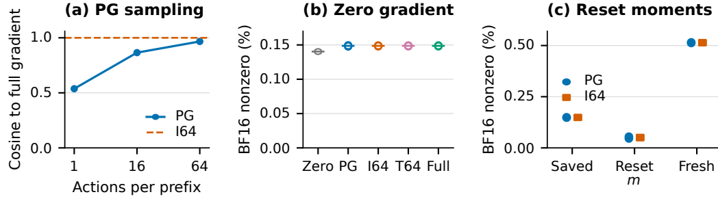
Figure 6: Averaging more token samples improves gradient alignment; Adam history contributes strongly to BF16 changes. (a) Gradient cosine to full-vocabulary supervision; I64 uses the top-64 intersection. (b,c) Fractions of changed BF16 weights with zero current gradient or reset moments. PG denotes sampled-token supervision; reset- m keeps the second moment and step count, and fresh Adam resets both moments and the count. Points show batches and bars show means.
