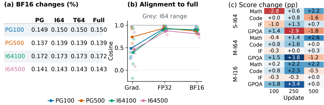
Figure 4: Top-64 supervision closely approximates the full-vocabulary gradient in Qwen and produces task-dependent learning gains. (a) Fraction of changed BF16 weights for each local loss at fixed checkpoints. (b) Gradient and update cosines to full-vocabulary supervision. (c) Score differences from sampled-token supervision over training. PG: sampled token; I16/I64: student-teacher top-16/top-64 intersection; T64: teacher top-64. S/M denote mathematics-only/joint training; checkpoint numbers are training updates.
