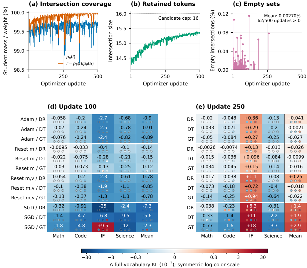
Figure 13: High average coverage and low mean probe loss can conceal exceptions. (a–c) I16 per-update means of 16 logged slices, without temporal smoothing; the mass axis spans 98.5–100%. (d,e) Full-vocabulary KL after minus before BF16 writeback, in units of 10^{-3} . Cells show three-batch means; dots show batches 1042–1044 from left to right. The shared symmetric-log color scale is linear within \pm 0.1 . SGD is matched to each rule’s Adam step norm.
