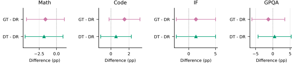
Figure 7: I64 averaging rules produce task-dependent score differences . Update-500 differences from DR (mean \pm std).
