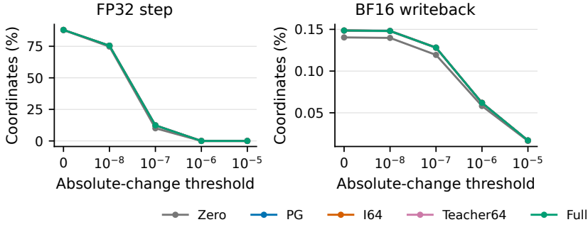
Figure 8: Update sparsity depends on the numerical threshold. FP32 steps and BF16 parameter changes; lines show batch means and shading their range.
