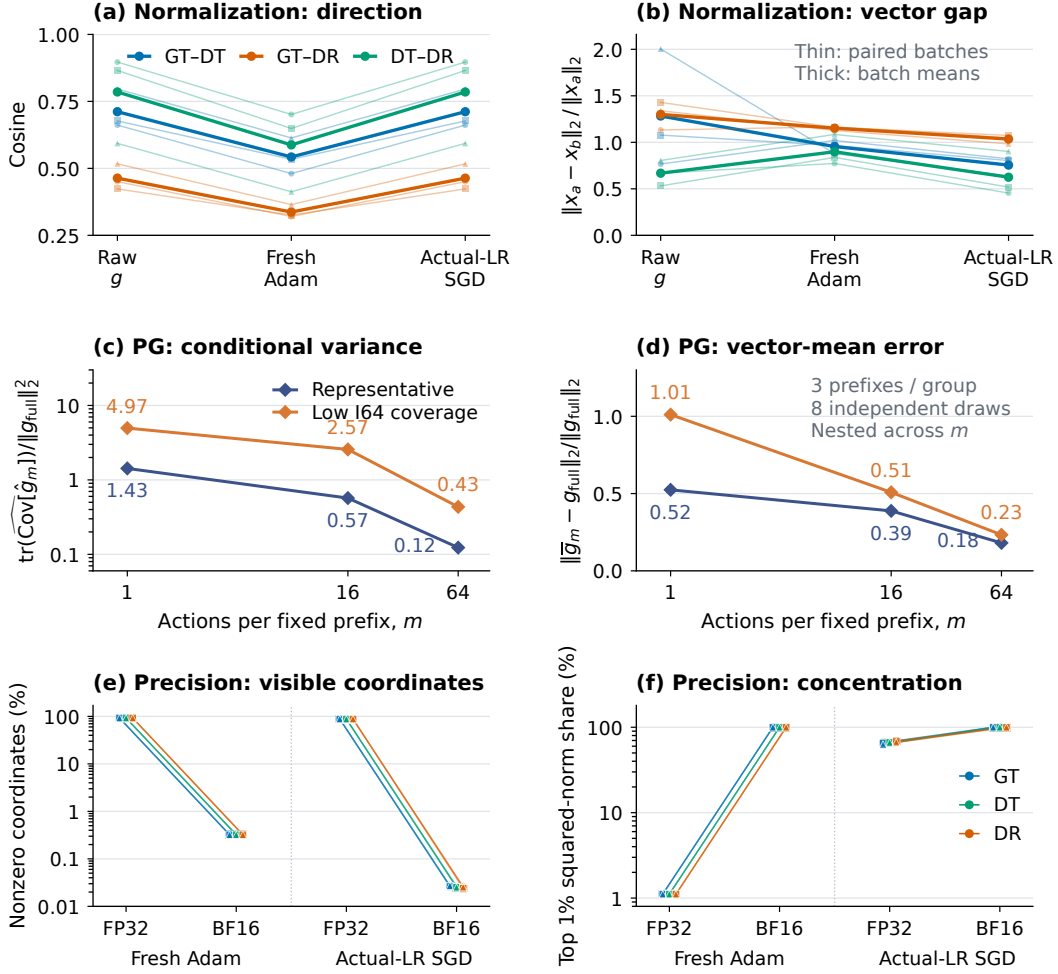
Figure 14: Local controls separate optimizer, sampling, and precision effects. (a,b) Three paired SmolLM3 batches (thin) and their means (bold). In (b), x is the gradient or step, normalized by the first named rule. (c,d) Three fixed prefixes per group, eight action repeats; (d) error of the vector mean. (e,f) Each rule/batch pairs FP32 changes with BF16 writeback. Fresh Adam uses zero moments at exported BF16 parameters, not native master weights or trained history.
