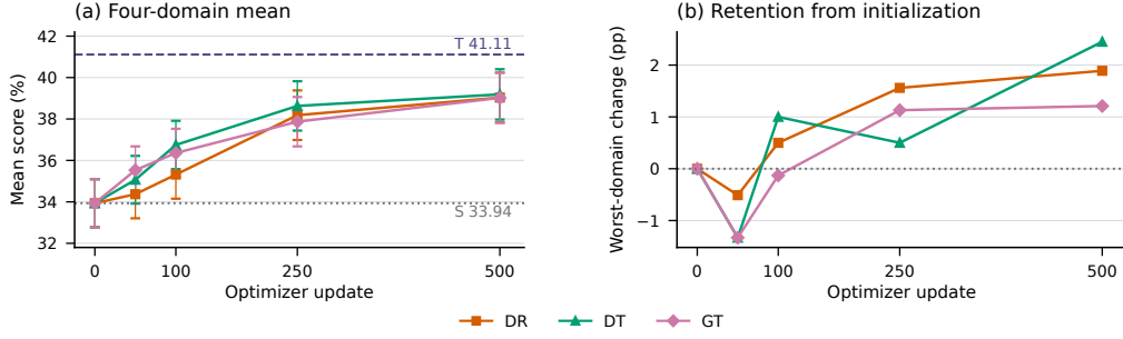
Figure 10: Mean performance gains can coexist with a regression in an individual domain. (a) Four-domain mean \pm std; S/T mark the initial student/teacher. (b) Worst-domain change from initialization; zero means no regression. Lines connect reported point estimates.
