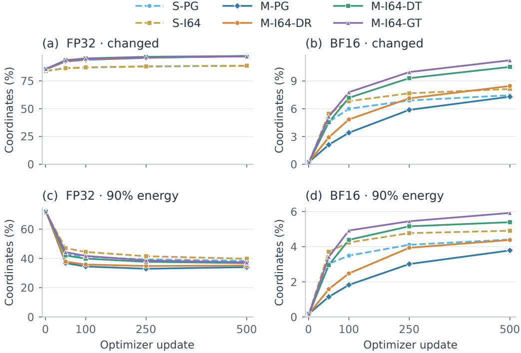
Figure 11: Cumulative BF16 changes remain much sparser than FP32 changes. PG/I64 trajectories under DR in single-teacher (S) and joint (M) training, with joint I64-DT/GT added: (a,b) nonzero coordinate fractions; (c,d) coordinate fractions containing 90% of squared displacement from initialization. Lines connect measured updates 1, 50, 100, 250, and 500; dashed lines denote S. No training-seed uncertainty is estimated.
