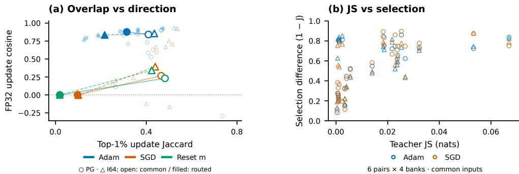
Figure 12: Coordinate overlap and update direction measure different properties. (a) Top-1% FP32 update-set Jaccard versus cosine; small/large points show batch/overall means. (b) Teacher-distribution JS divergence versus 1-Jaccard on shared inputs; each point is a teacher pair within a batch.
