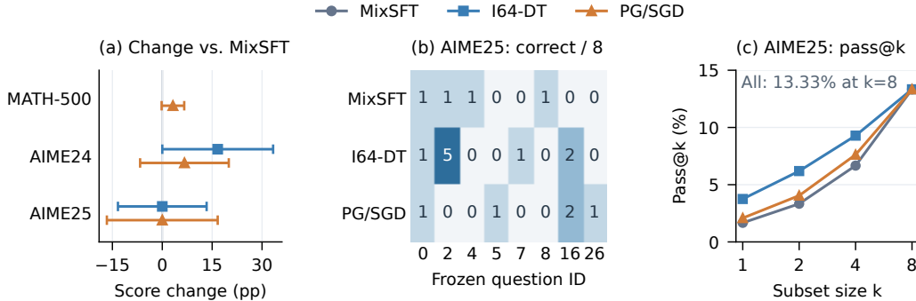
Figure 16: Equal aggregate scores can conceal different solved questions and sampling outcomes. (a) Differences from MixSFT with paired question-bootstrap 95% intervals: accuracy for MATH-500, pass@8 for AIME. (b) Correct responses out of eight for every AIME 2025 question solved by any model; the other 22 questions have zero successes. (c) Subset estimates from the same eight responses: \widehat{\text{pass@}k} = \frac{1}{30} \sum_q [1 - \binom{8-c_q}{k} / \binom{8}{k}] , where c_q counts correct responses.
