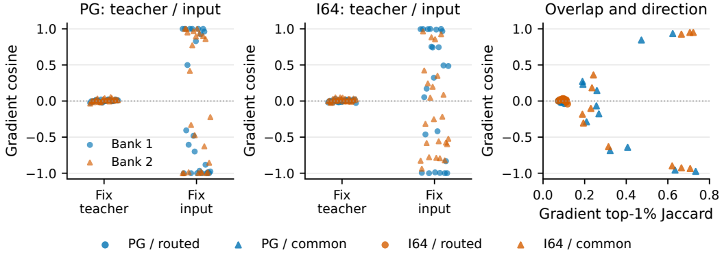
Figure 9: Gradient overlap depends strongly on the input domain. Left/center: teacher-by-input-domain controls. Right: top-1% gradient Jaccard versus cosine on domain-specific or shared inputs.
