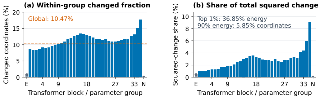
Figure 15: Cumulative BF16 changes differ across all 38 SmolLM3 parameter groups. MixSFT to DR500: blocks 0–35, embedding (E), final norm (N). (a) Within-group changed fraction; dashed: global parameter-weighted fraction. (b) Share of total squared displacement. Tied weights count once; native FP32 changes are unavailable.
