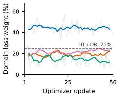
(a) Domain weights
