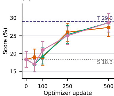
(e) IFBench strict
