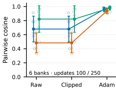
(b) Gradient to update
