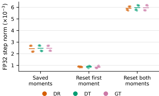
Adam memory sets the step size
