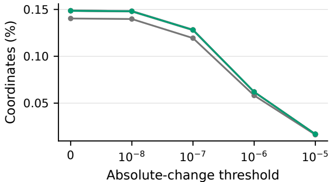
BF16 local writeback
