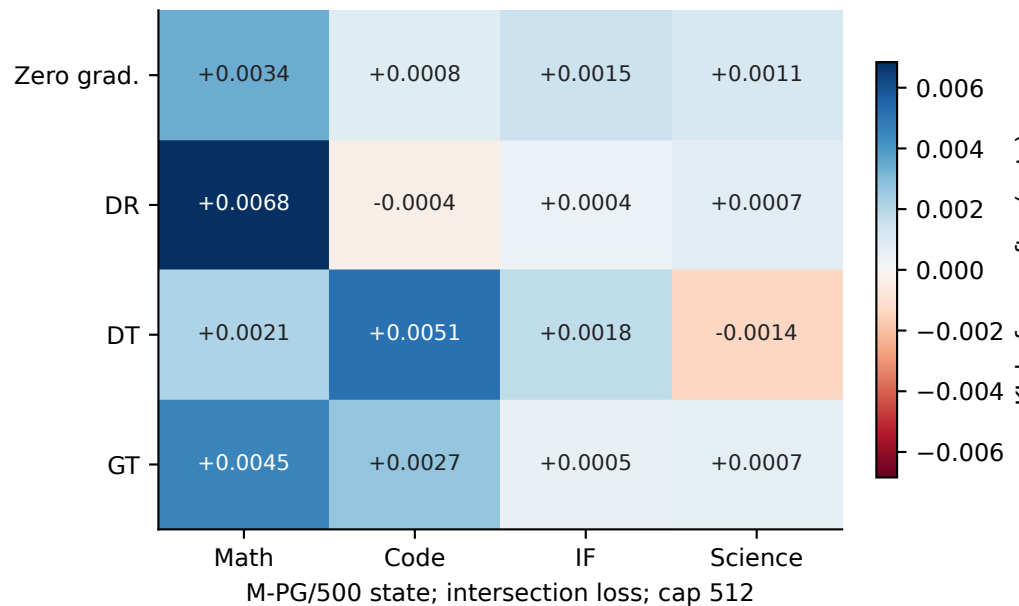
F2c Local held-out KL decrease
