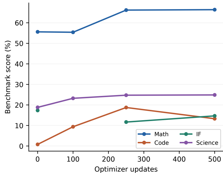
F8b (partial) M-PG capability
