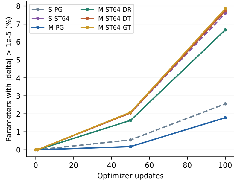
F4a (partial) Cumulative BF16 changes
