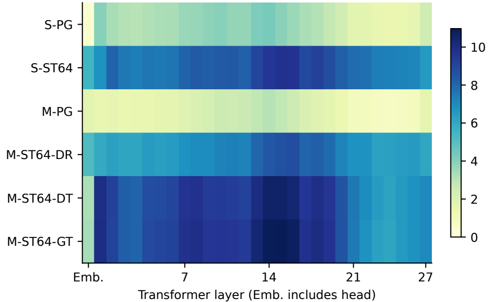
F4c (partial) Layer concentration at 100
