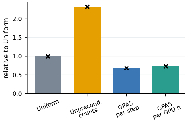
Preconditioned gradient variance
