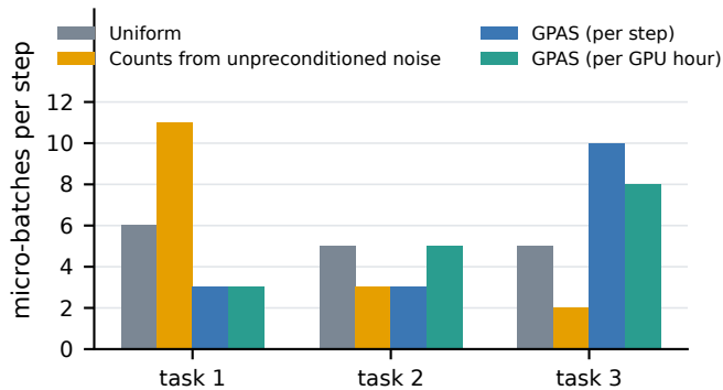
Integer micro-batch allocation
