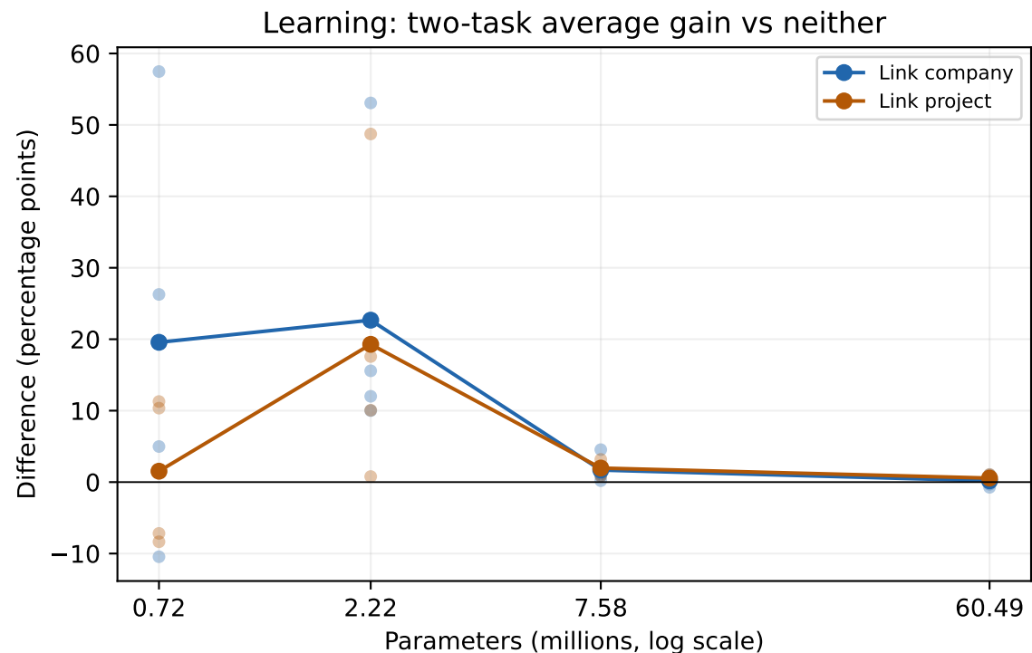
Paired effects across model sizes Dots: four world/initialization blocks; lines: means
