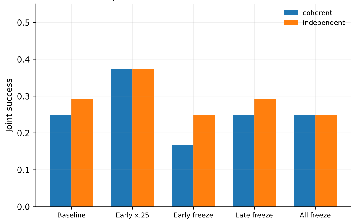
Development interventions: fixed Adam editor
