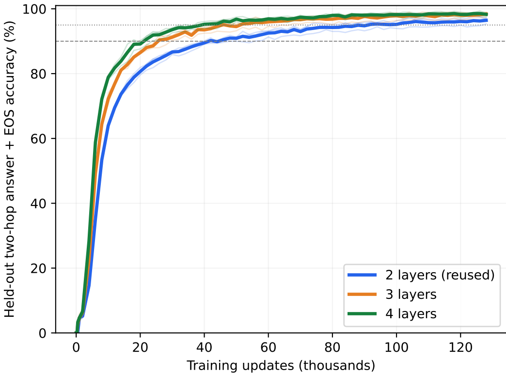
Paired depth extension: 3 worlds, 2 initializations per world
