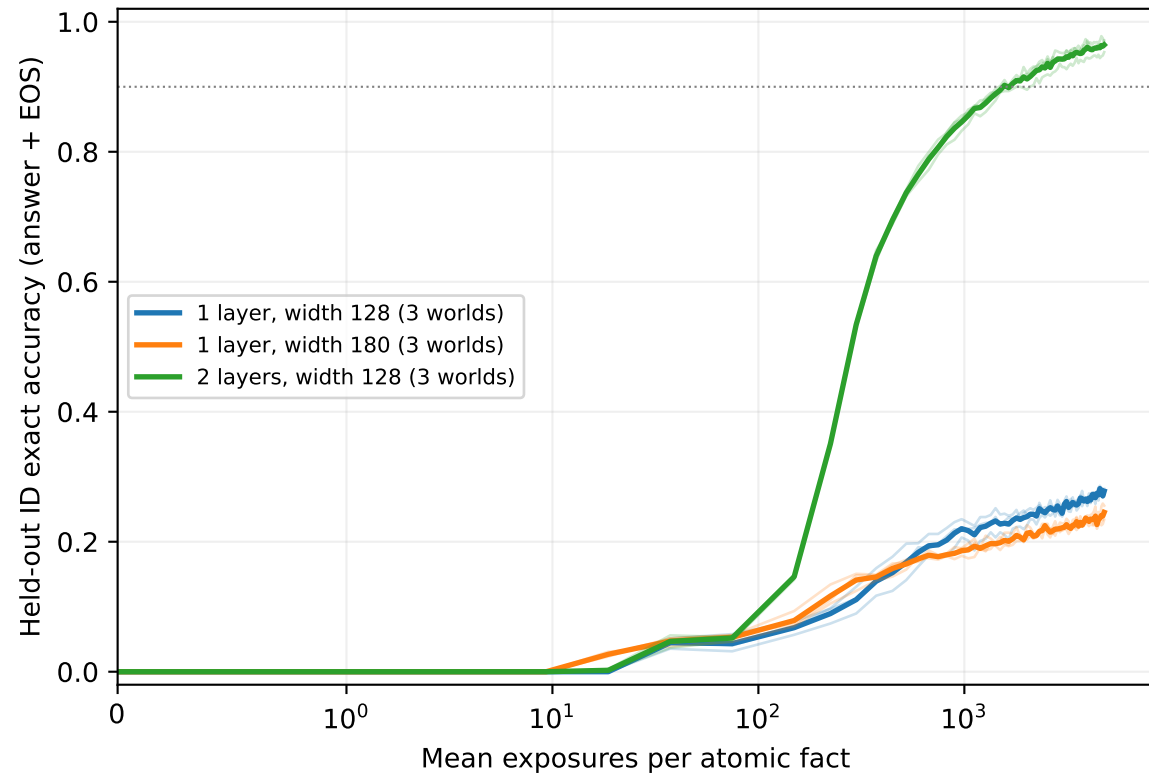
Two-hop generalization across 3 independent worlds
