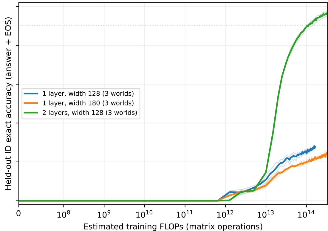
Two-hop generalization across 3 independent worlds
