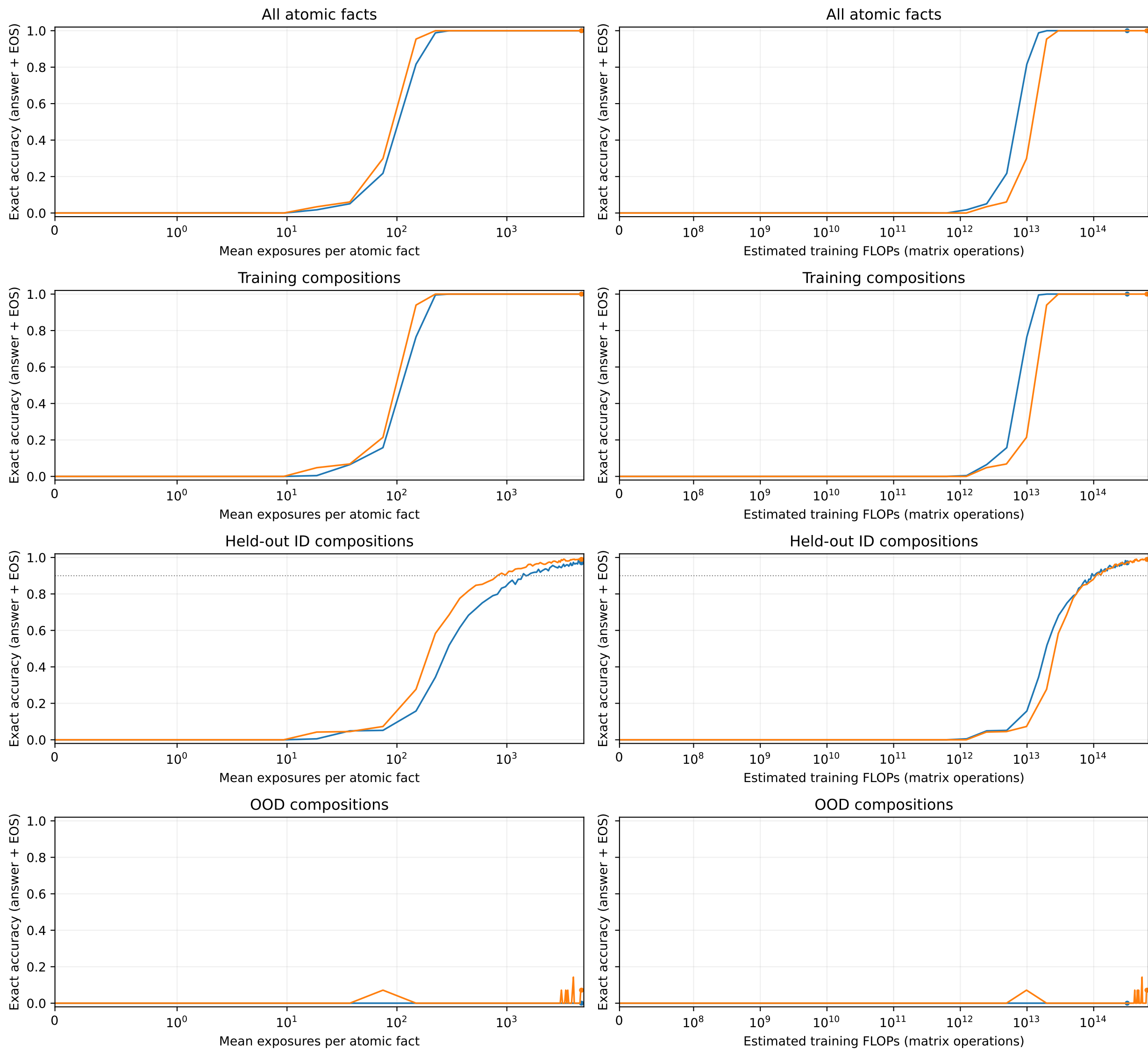
Development: individual learning curves; incomplete runs are dashed
